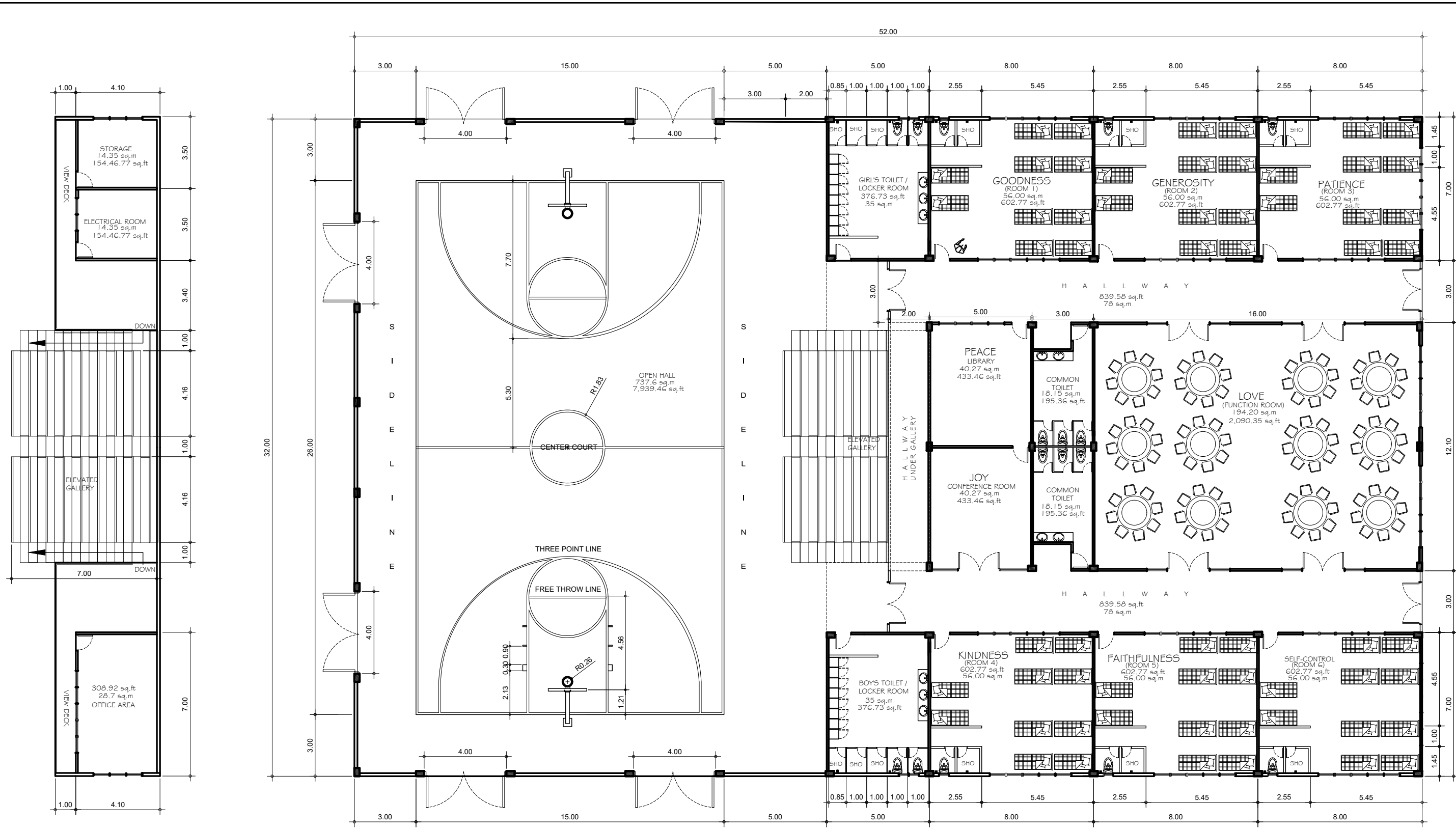
TOTAL FLOOR AREA 1669.199 SQ.M FLOOR PLAN
